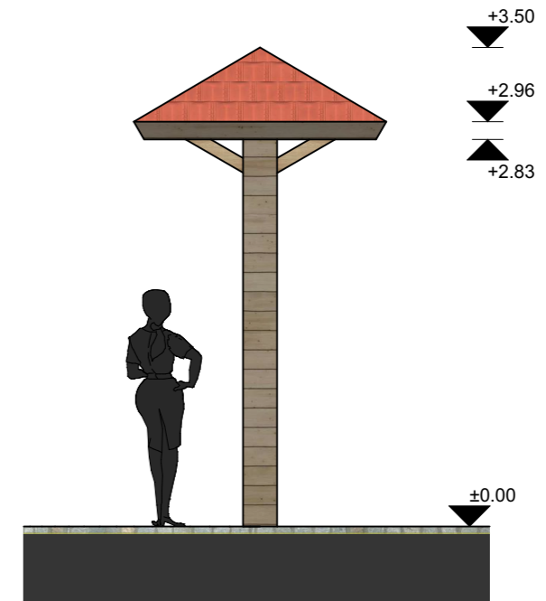
FATADA LATERALA
