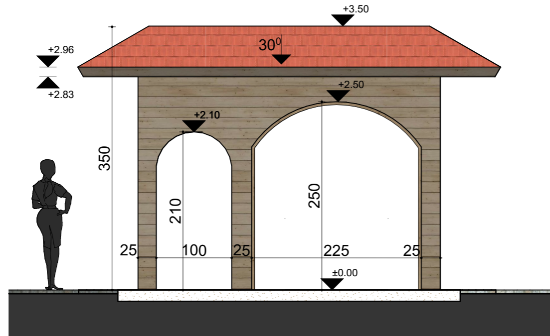
FATADA PRINCIPALA
