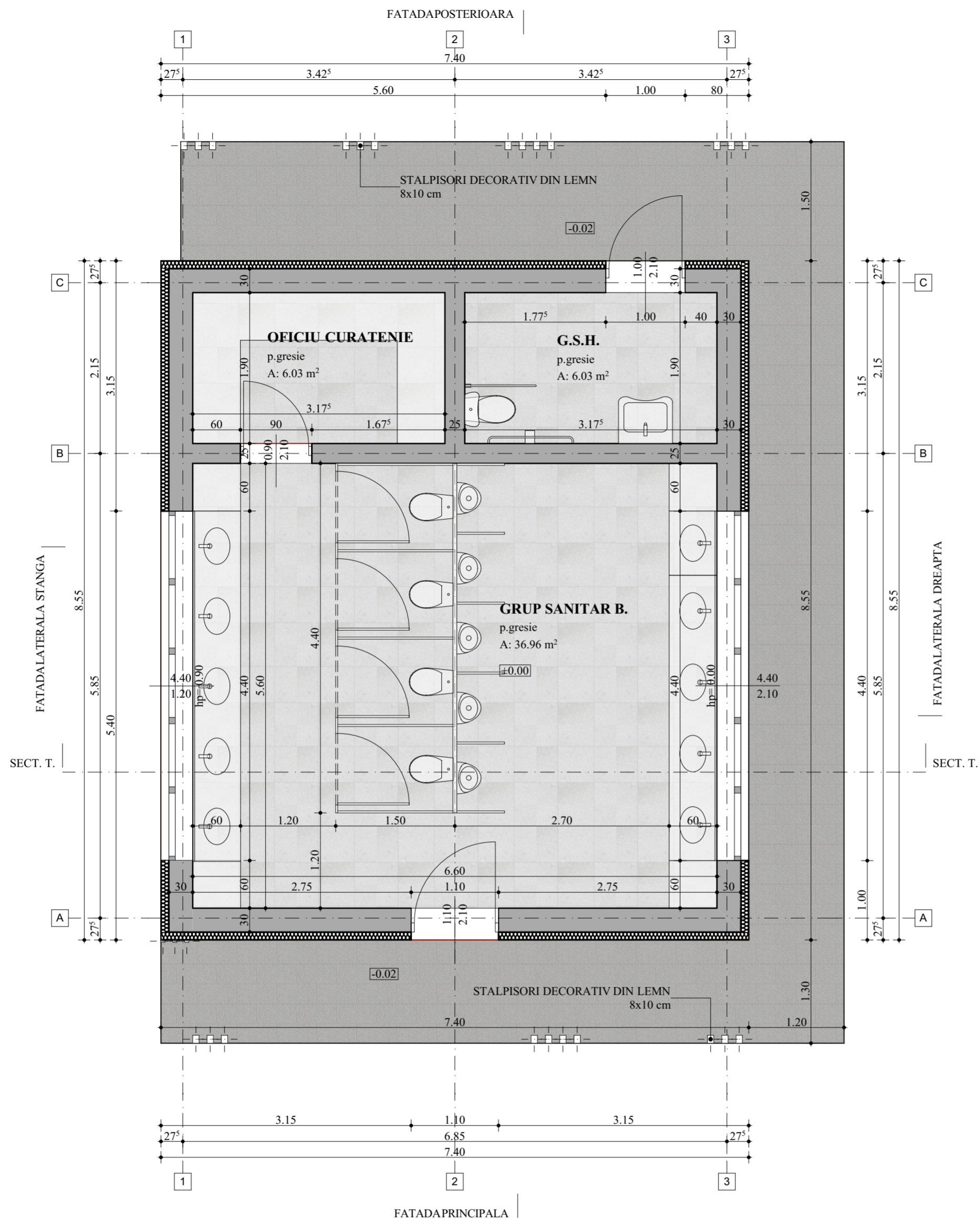
PLAN PARTER
